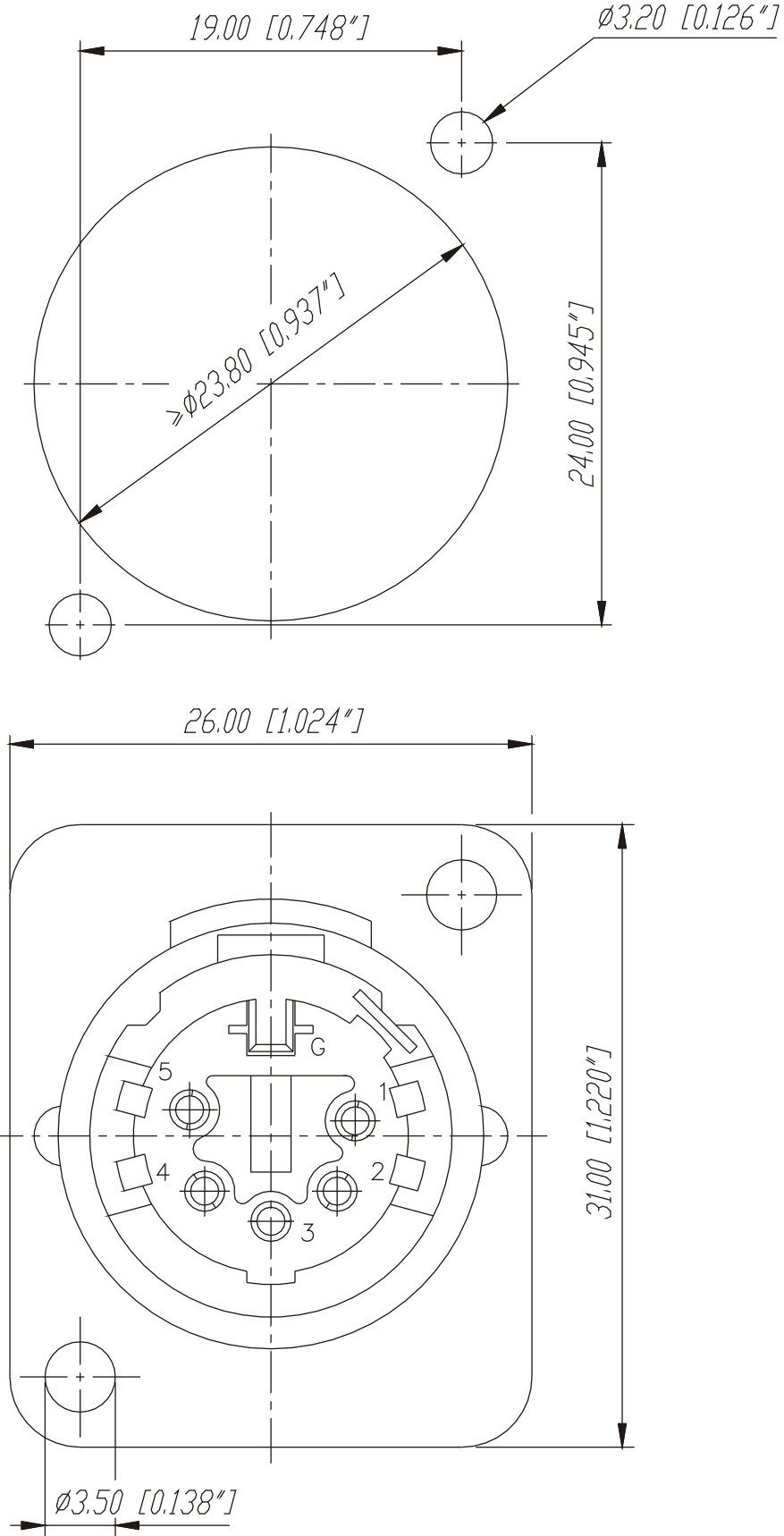
Panel cut out (rear side)
