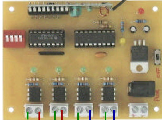
RF 4Channel Receiver / SW Board
