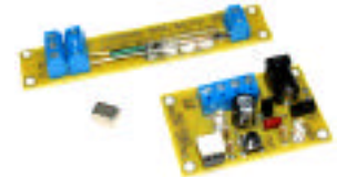
Latching Reed Switch (BPE # LRS-0075)
